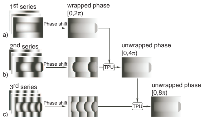
Fig. 20 Temporal phase unwrapping: a) a series of phase-shifted images is projected with a projected wavelength P_{p1} longer or equal to the plane length. \phi_1 is equal to the unwrapped phase \varphi_1 . b) a second series of phase-shifted images is projected, but with a wavelength P_{p2} set to half the length P_{p1} . \phi_2 is computed. The unwrapped phase \varphi_2 is directly calculated by adding 0 or 2\pi to \phi_2 so that \phi_2 + (0or2\pi) = 2\phi_1 + \epsilon . c) This processes is repeated with a new series of images.
