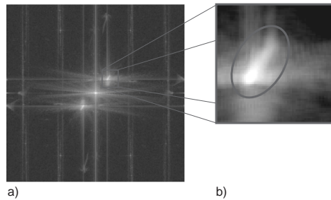
Fig. 10 Image in the FFT domain with the frequency f_0 of the projected fringe in a nontelecentric setup: a) overview, b) close-up of the diffuse peak F_\phi
