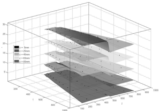
Fig. 18 Calibration matrix M_{ij\varphi} with five reference planes z - k . The dots represent the position of the circle centers on the calibration plane.
