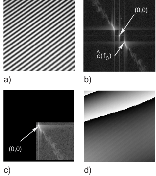
Fig. 7 Reference plane: a) projected fringes, b) image in FFT domain with the frequency f_0 of the projected fringe, c) image filtered and shifted and d) reference plane phase map.
