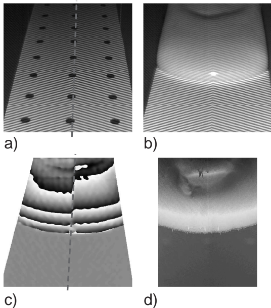
Fig. 19 Projection of a symmetric pattern not aligned with the reference plane, a) grabbed image of the reference plane with the axis of symmetry in the dotted line, b) grabbed image of the sluice, c) phase map with a step on the axis of symmetry, d) the resulting surface without any step.
