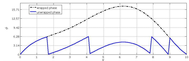
Fig. 13 Example of phase unwrapping in 1D.
