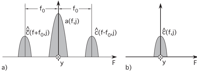
Fig. 6 Frequency map: a) of a grabbed image, b) with only the frequency of the projected cosine shifted to zero.
