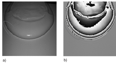
Fig. 9 Fringe projection at 45°: a) grabbed image, b) phase map computed with FTP. The phase map exhibits erroneous frequencies on the bottom left corner (area marked with the ellipsis).
