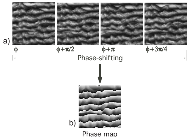
Fig. 5 Phase shifting: a) with 4 images and b) the resulting phase map.
