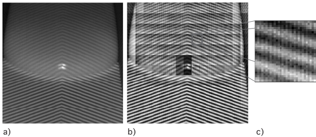
Fig. 11 a) grabbed image, b) local wave retrieval using window, c) close-up of one window.
