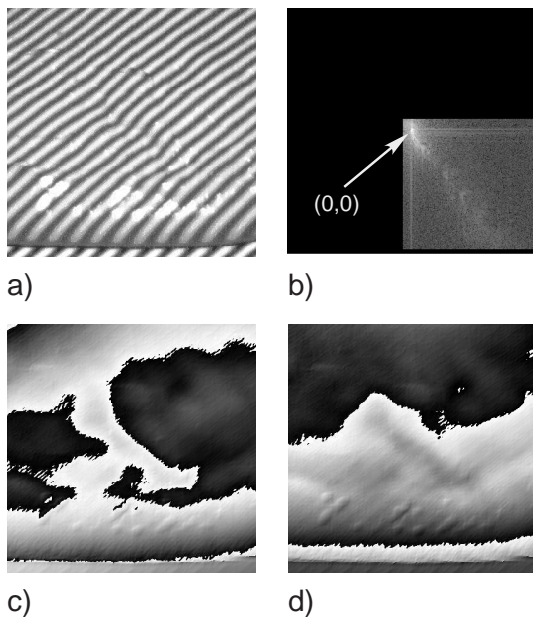
Fig. 8 Object: a) projected fringes, b) object image filtered and shifted in Fourier domain c) resulting phase map, and d) difference between the object phase map and the reference plane phase map.
