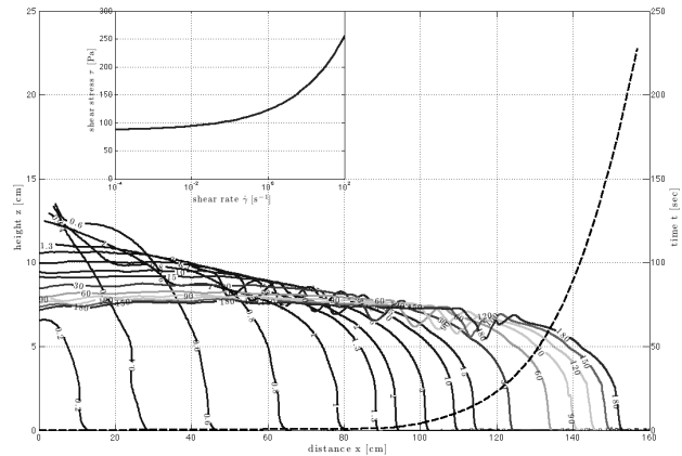
Fig. 22 Mid-profile of the surge (continuous lines) and position of the front in function (dash line) of the time for a visoplastic fluid with a yield stress of 86 [Pa]
