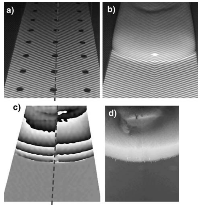
Fig. 19 Projection of a symmetric pattern not aligned with the reference plane; a grabbed image of the reference plane with the axis of symmetry in the dotted line, b grabbed image of the surface, c phase map with a step on the axis of symmetry, d the resulting surface without any step
