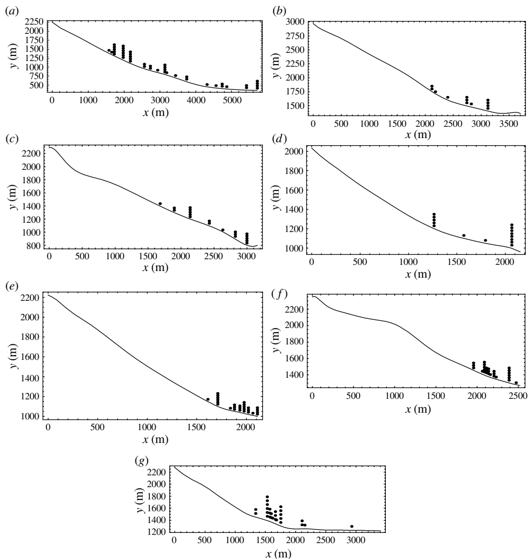
Figure 2. Regularized path profiles. Each dot represents a recorded run-out distance. (a) Saint Clément path, (b) Gurrasz path, (c) Scey path, (d) Saugy path, (e) Chantey path, (f) Nants path.
