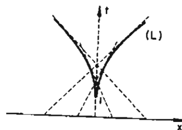
Figure 5 u_0 = -\tanh x (L): t = \text{Ch}^2 \xi x = \xi - \text{Sh} \xi \text{ Ch} \xi
