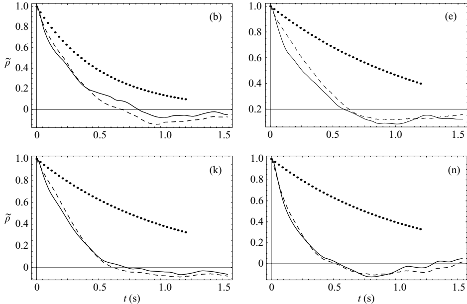
FIGURE 8. Autocorrelation functions of the number of moving beads (solid line) and the solid discharge (dashed lines). Dotted lines stand for the theoretical autocorrelation function (2.22), when the autocorrelation time \hat{t}_c is evaluated using (4.1). Experiments (b), (e), (k) and (n).
